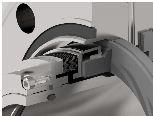
Outward-pumping spiral groove and HTC Technology
