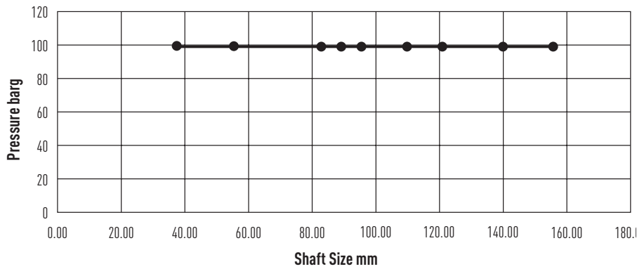
Type 8648VRS Basic Pressure Rating, Crude Oil
